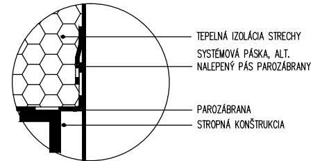
DETAIL III
